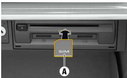
Fig. 1: Inserting external SIM card in glove box and removing
