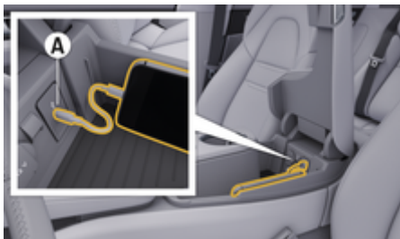
Fig. 3: USB interface (Type C) in armrest
